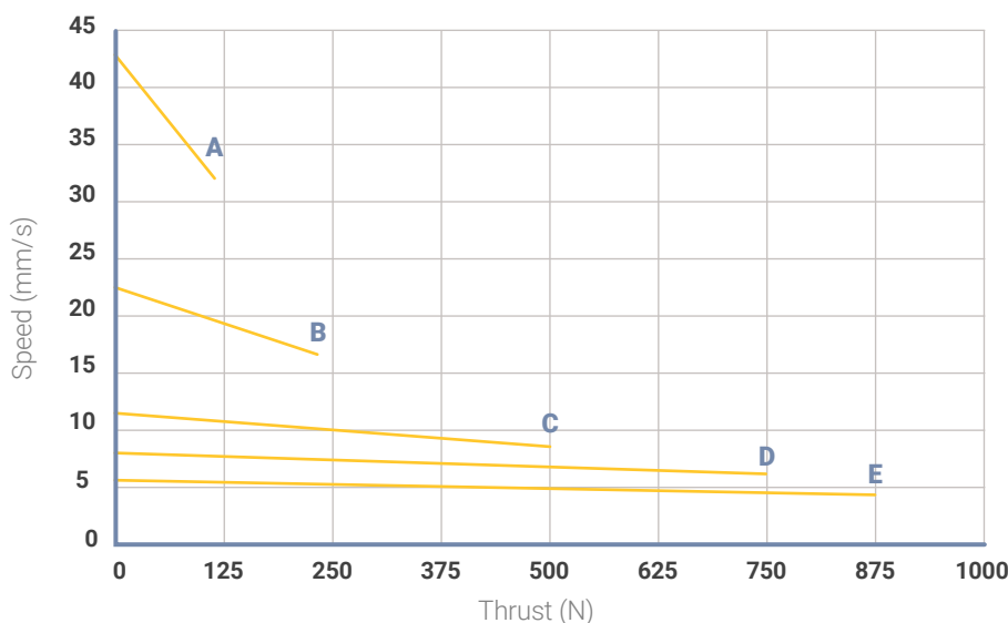
Speed vs. Thrust
