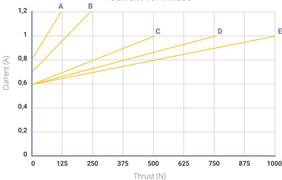
Current vs. Thrust
